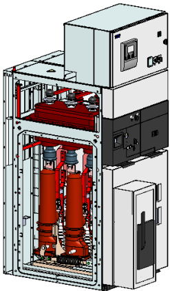
Circuit breaker panel Type CBFF
