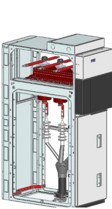
Ring-main panel Type SF
