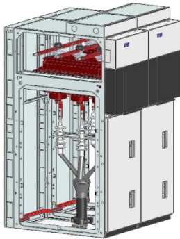
Bus sectionaliser panel Type BC2
